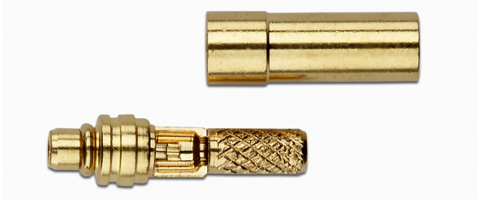
Model 73023 MMCX PLUG STRAIGHT CRIMP, RG174, 316
